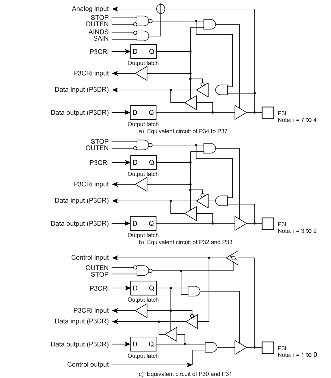
Figure 5-5 Port P3
