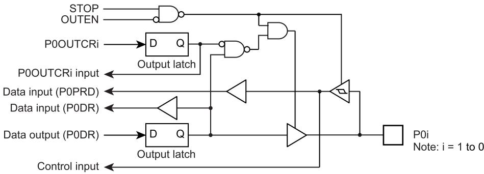
Figure 5-2 Port P0
