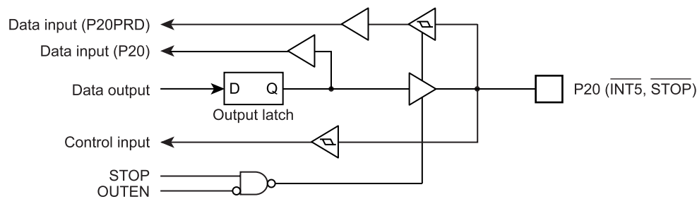
Figure 5-4 Port P2
