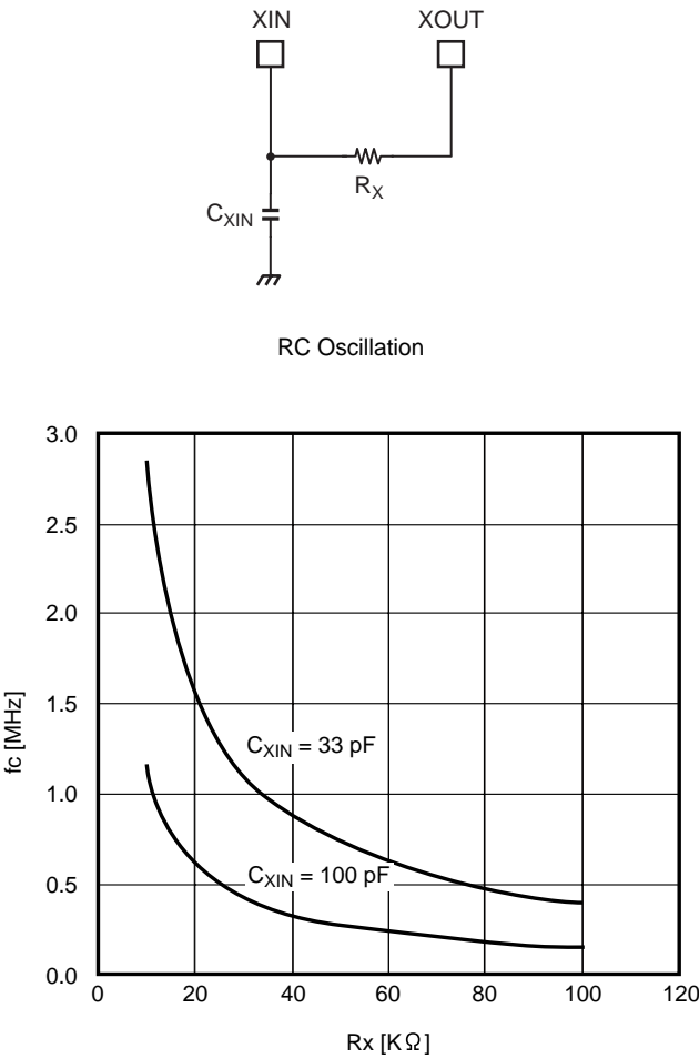
Figure 12-1 Oscillation Frequency (f c ) vs R x (V DD = 5.0 V, Ta = 25°C)
