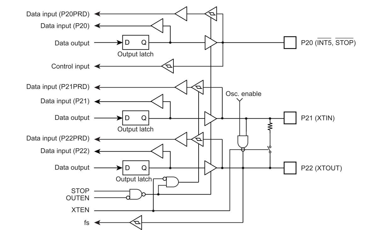
Figure 5-4 P2 Port
