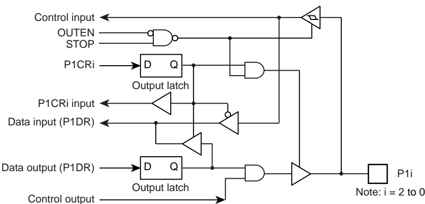
Figure 5-3 P1 Port
