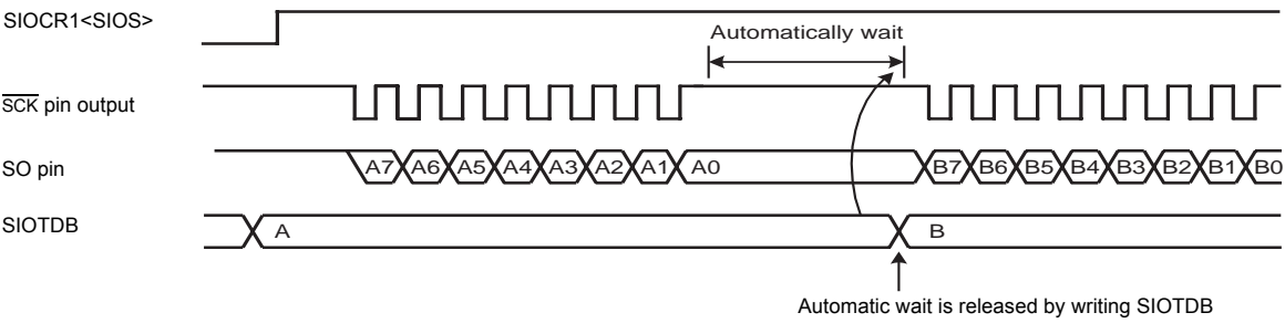
Figure 11-2 Automatic-wait Function (Example of transmit mode)
