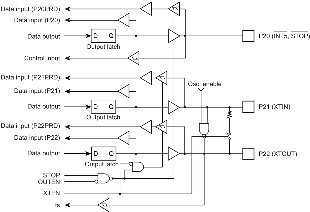
Figure 5-4 Port P2
