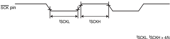
Figure 11-3 External Clock
