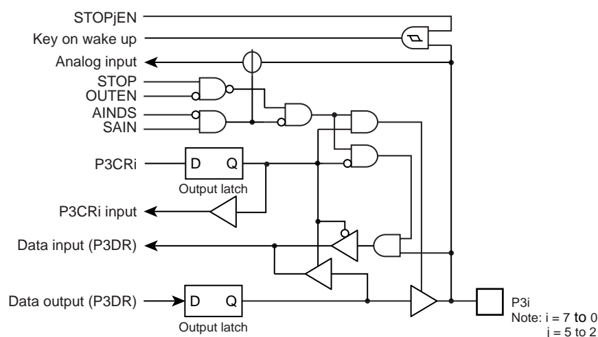
Figure 5-5 Port P3
