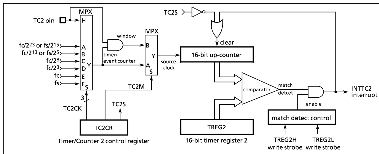
Figure 2-21. Timer/Counter 2 (TC2)
