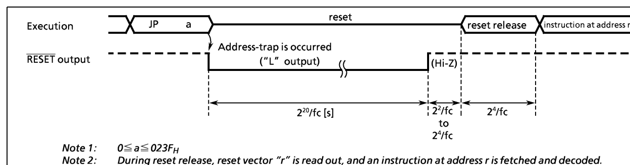
Figure 1-31. Address-Trap-Reset
