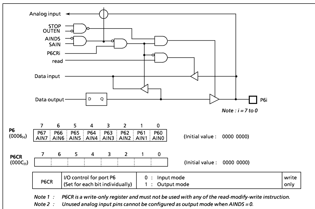
Figure 2-6. Port P6
