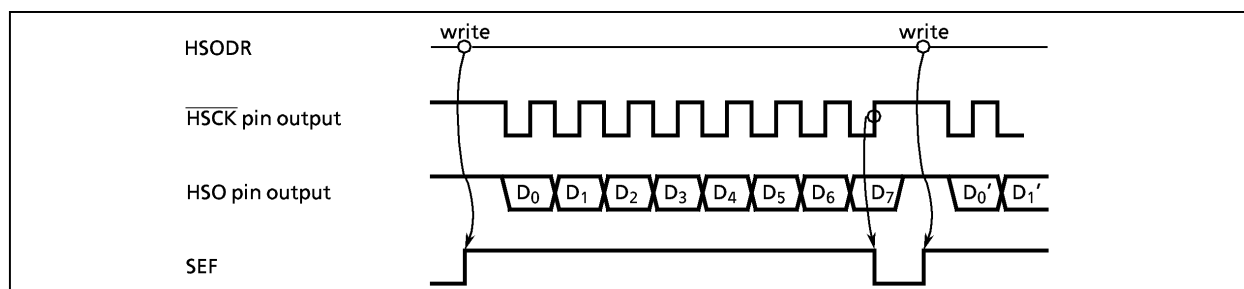
Figure 2-42. High-speed Serial Output Timing Chart
