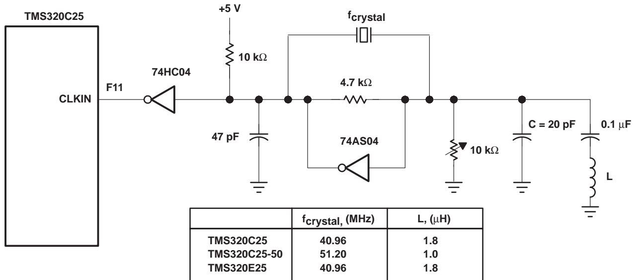
Figure 3. External Clock Option
