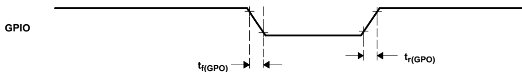
Figure 6-8. General-Purpose Output Timing
