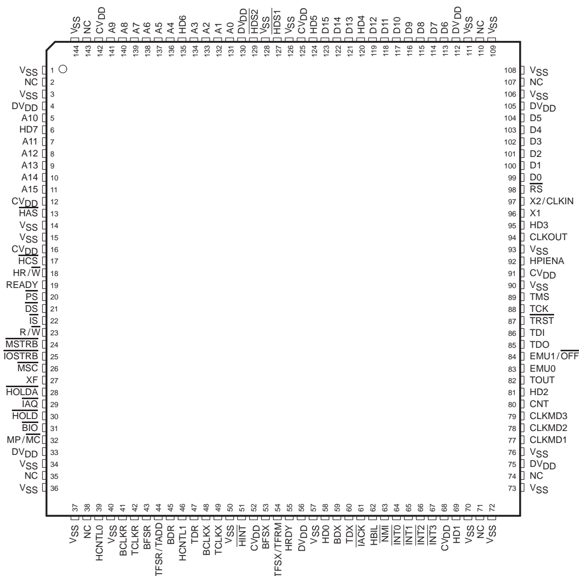
TMS320C542/TMS320LC542 PGE PACKAGE†‡ (TOP VIEW)
