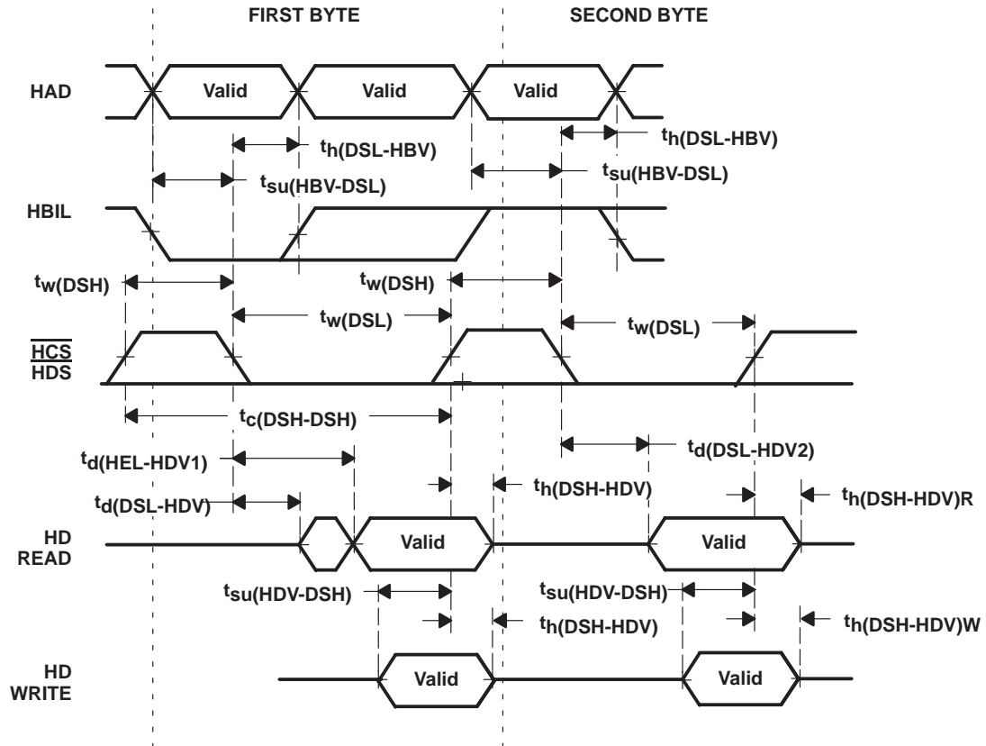
Figure 40. Read/Write Access Timings Without HRDY or \overline{HAS}
