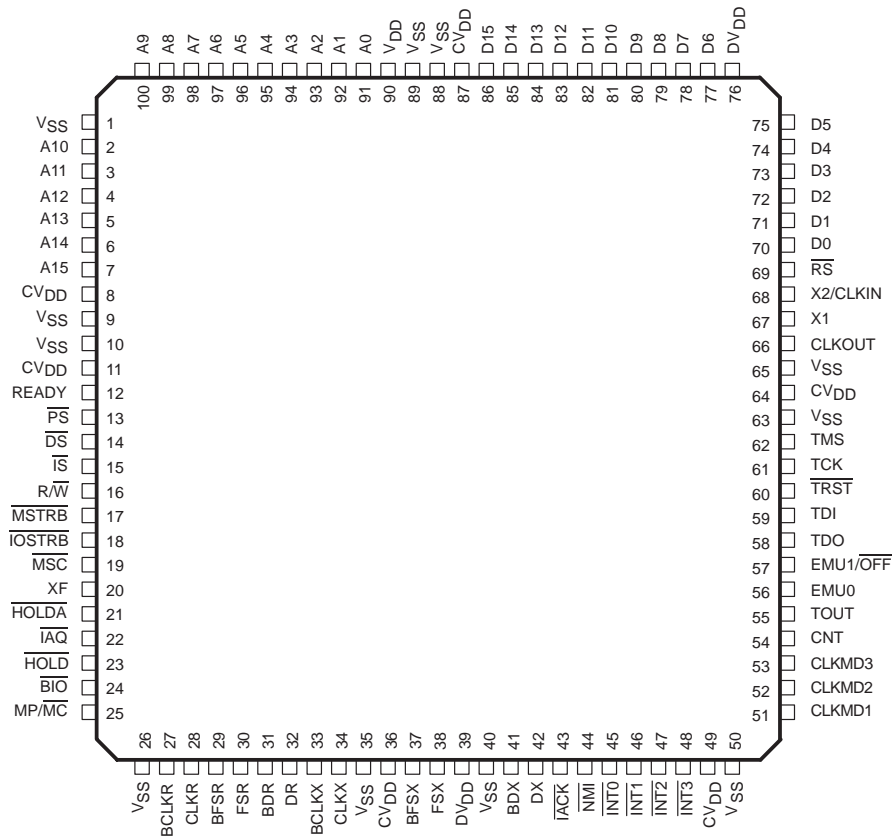
TMS320LC546 PZ PACKAGE† (TOP VIEW)
