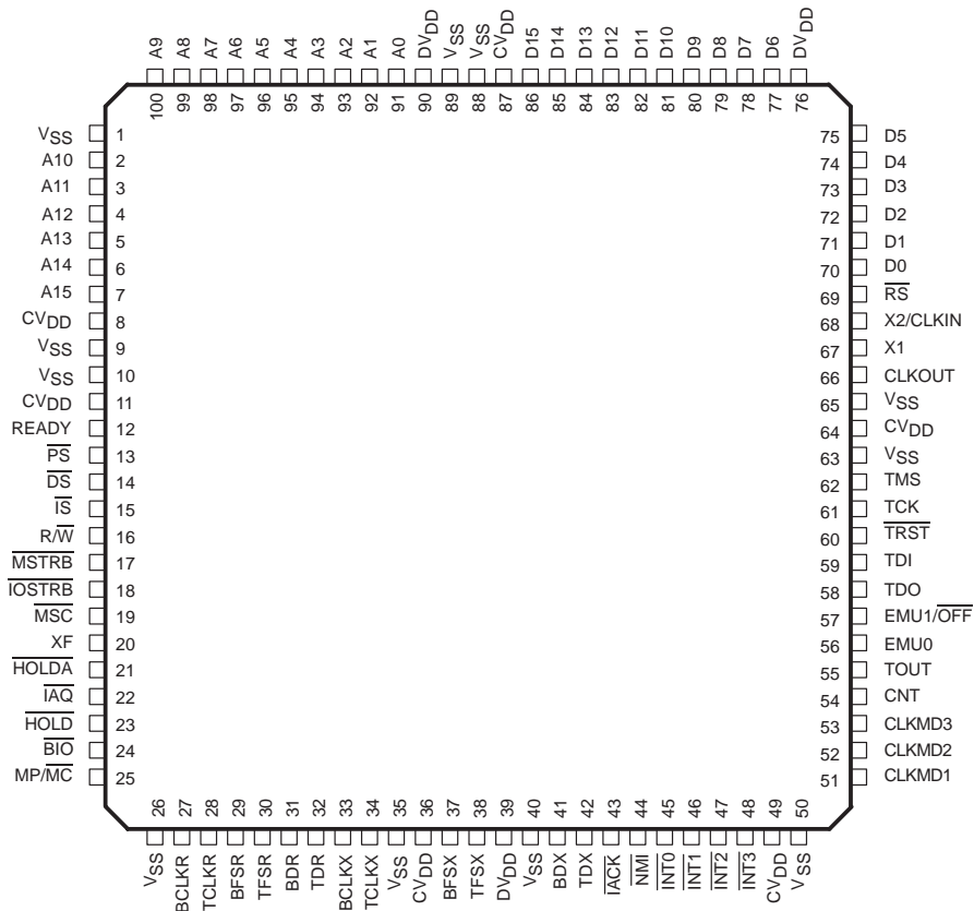
TMS320LC543 PZ PACKAGE† (TOP VIEW)
