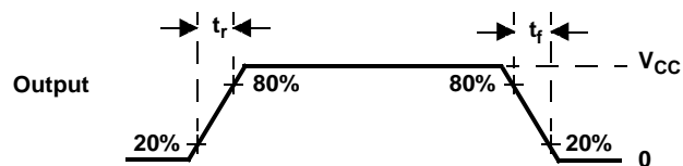
Figure 11. CMOS-Level Outputs
