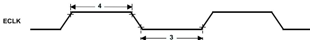
Figure 8. ECLK Timing Diagram
