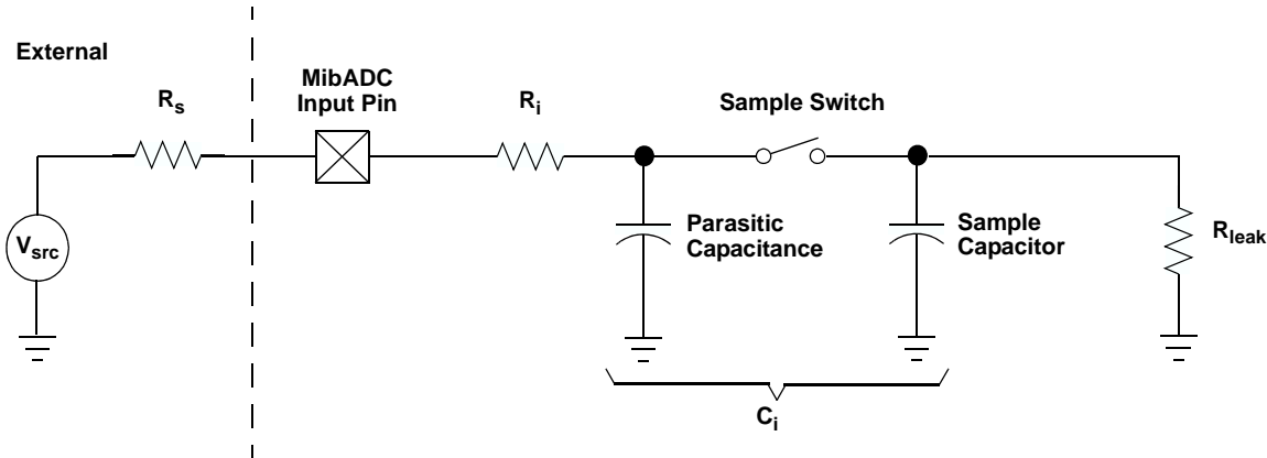
Figure 22. MibADC Input Equivalent Circuit
