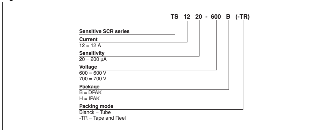
Figure 16. TS12 series
