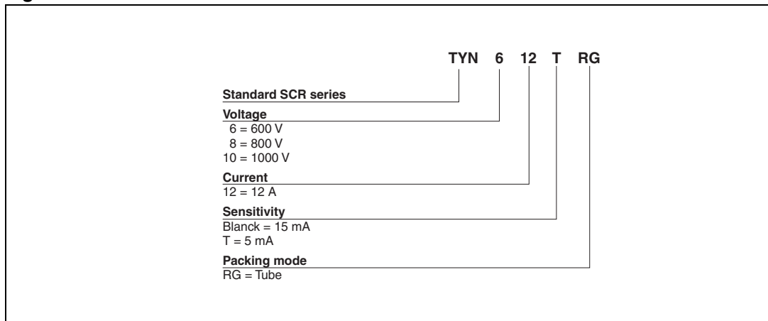
Figure 17. TYNx12 series
