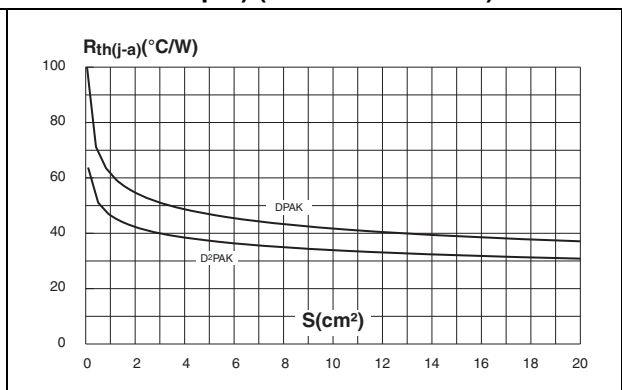
Figure 14. Thermal resistance junction to ambient versus copper surface under tab (epoxy printed circuit board FR4, copper thickness: 35 μm) (DPAK and D 2 PAK)
