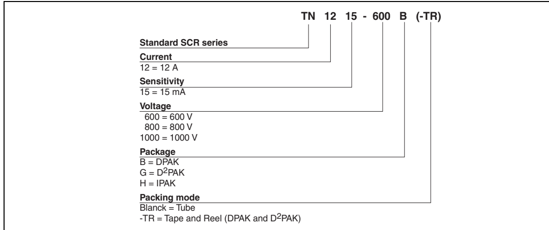
Figure 15. TN12 series
