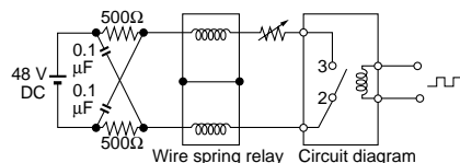
Circuit
