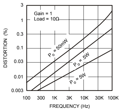
HARMONIC DISTORTION
