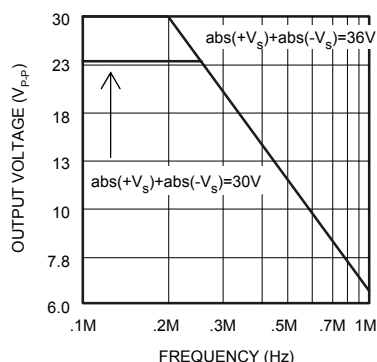
POWER RESPONSE
