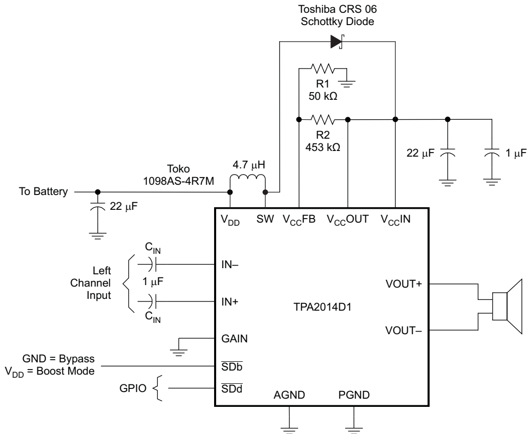
Figure 17. Bypass Circuit
