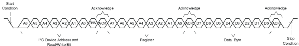
Figure 44. Single-Byte Write Transfer
