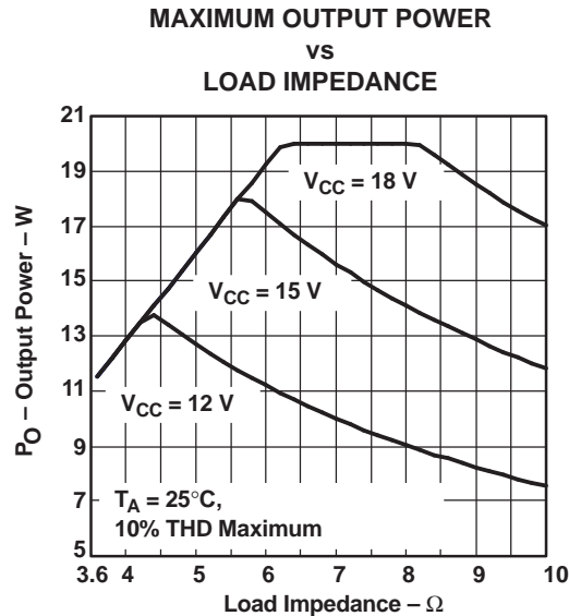
Figure 33. Output Power
