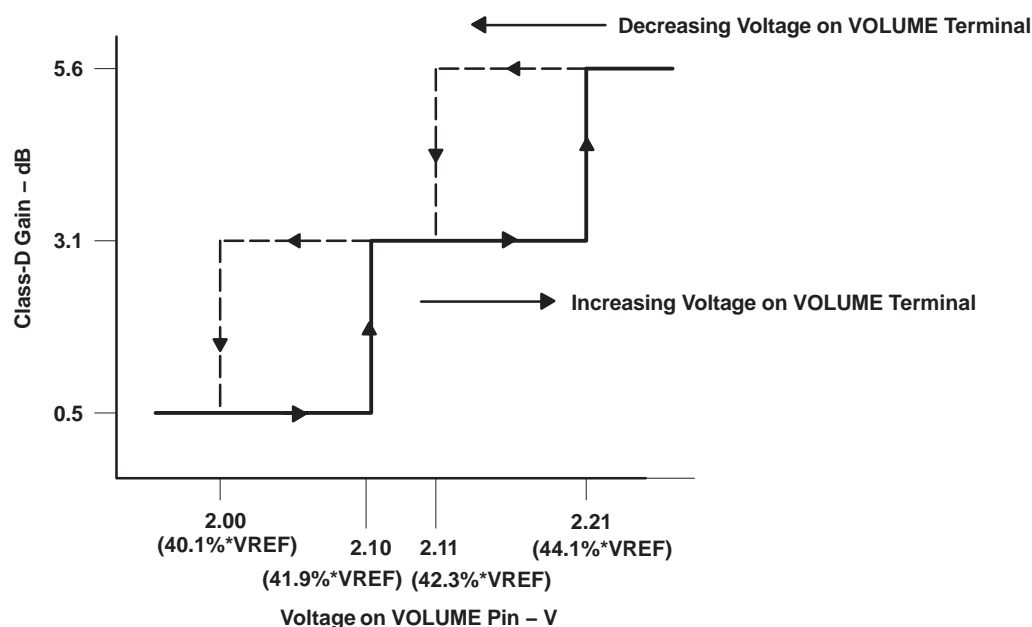
Figure 36. DC Volume Control Operation, VREF = 5 V
