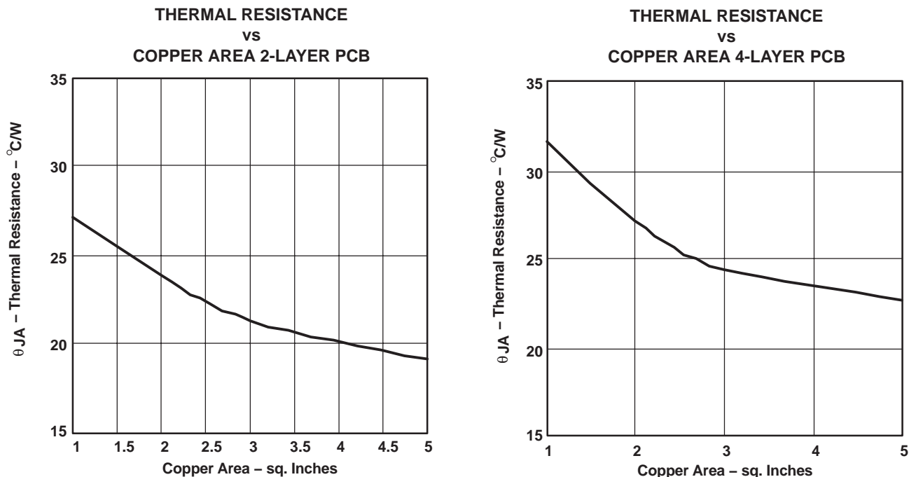
Figure 38. Thermal Resistance
