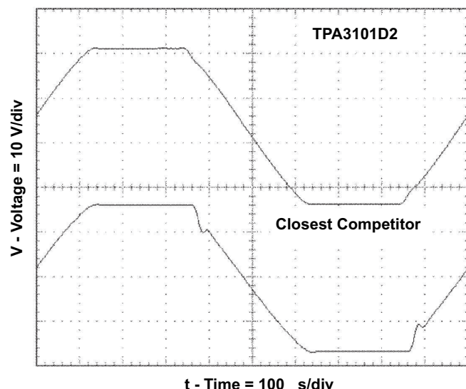
Figure 31. 1-kHz Sine Output at 10% THD+N
