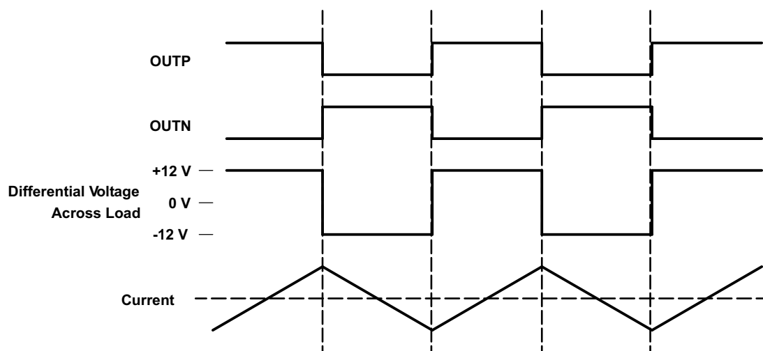
Figure 25. Traditional Class-D Modulation Scheme's Output Voltage and Current Waveforms into an Inductive Load With No Input
