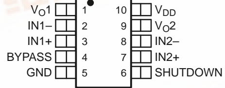
DGQ PACKAGE (TOP VIEW)
