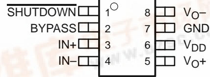
MicroStar Junior™ (GQS) Package (TOP VIEW)
