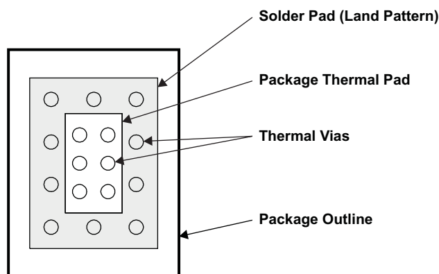
Figure 21. Package and PCB Land Configuration for a Multilayer PCB
