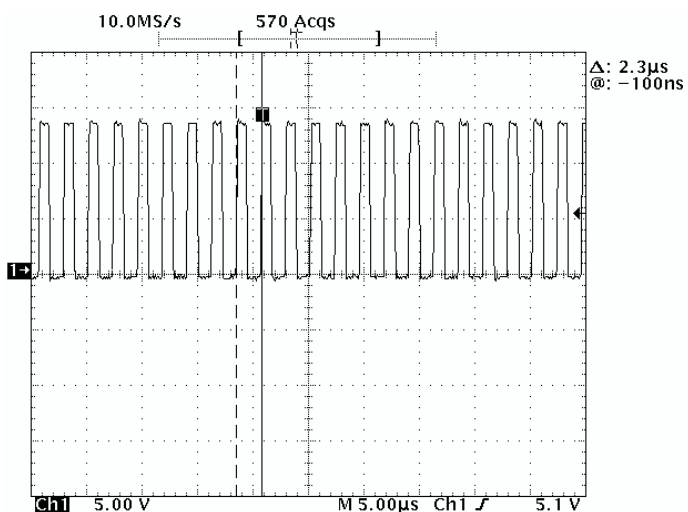
Figure 12. Nominal Switching Frequency of Q1 Switch (446 kHz)
