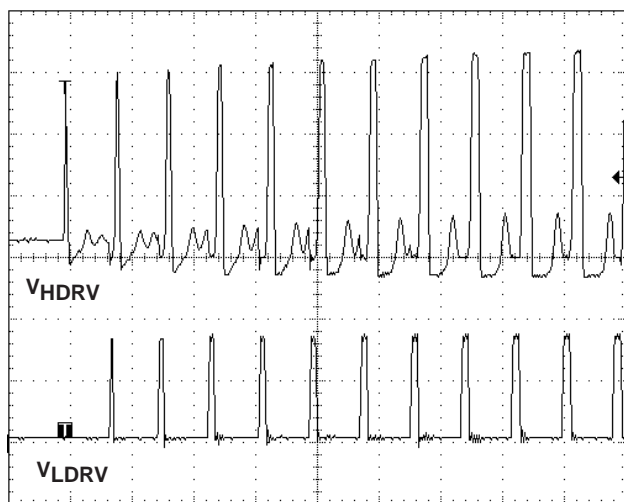
t – Time – 2 μs/div
