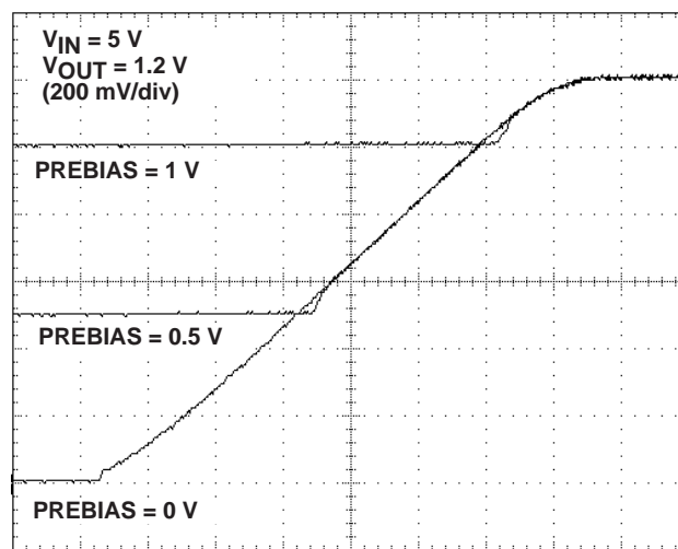
t – Time – 500 μs/div
