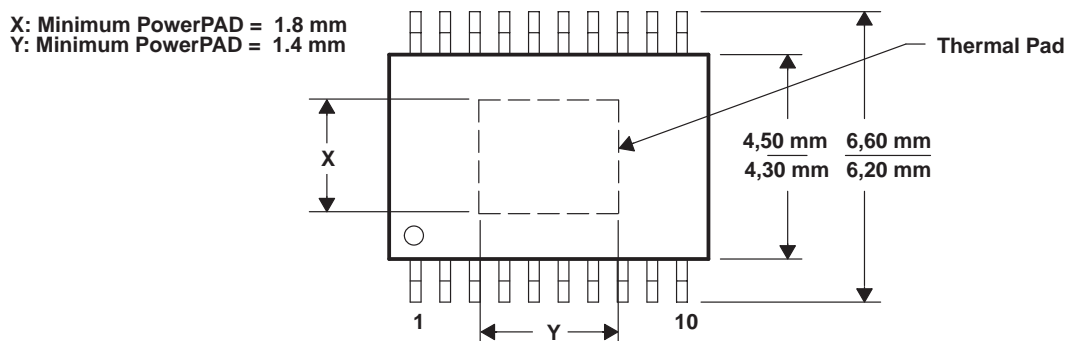
Figure 10. PowerPAD Dimensions
