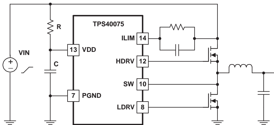
Figure 25. Limiting the Slew Rate
