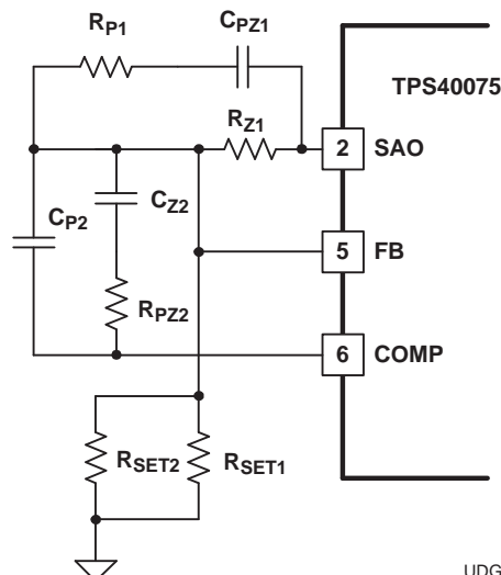
Figure 31. Type III Compensation with TPS40075
