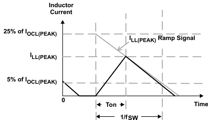
Figure 43. Inductor Current Limit at Pulse Skipping
