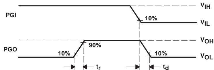
Figure 5. PG Output Voltage Waveform
