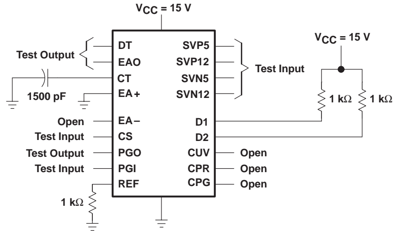
Figure 1. Test Circuit
