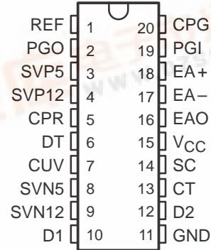
N PACKAGE (TOP VIEW)
