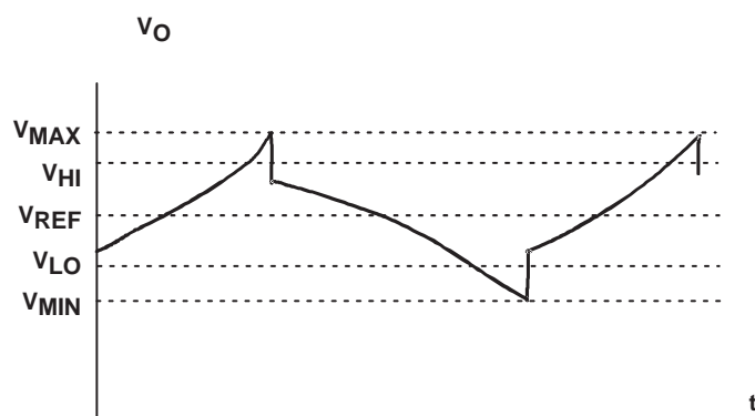
Figure 20. Output Ripple
