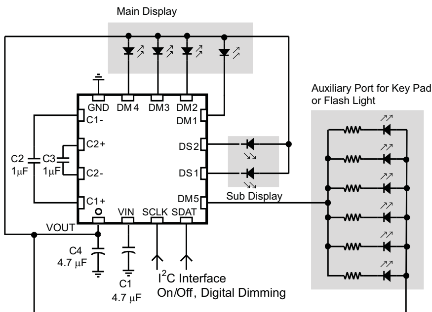
Figure 21. The Typical Application Circuit for Sub, Main, and Keypad Backlight
