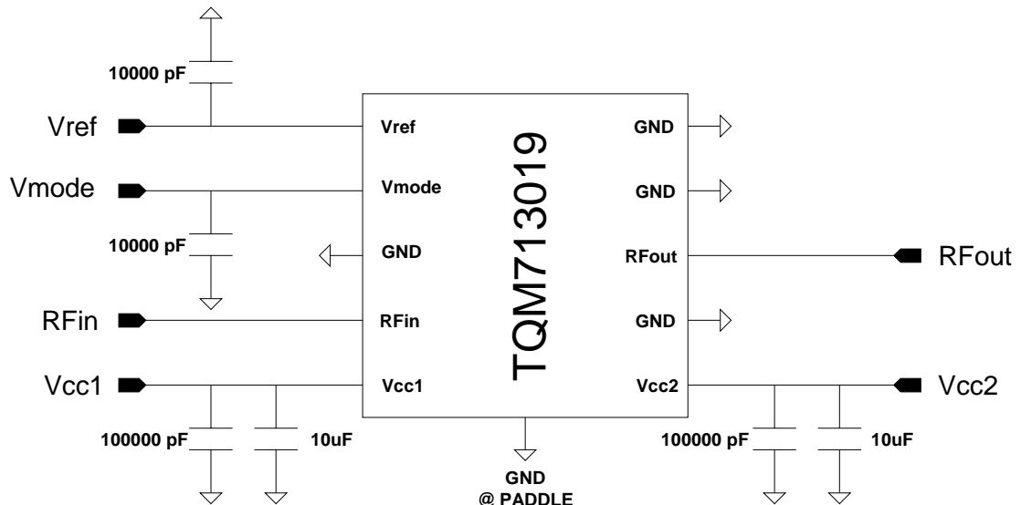
Figure 2: Evaluation Board Schematic
