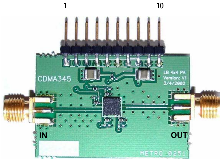
Figure 1: Evaluation Board
