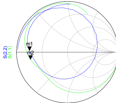
freq (30.00MHz to 6.000GHz)
