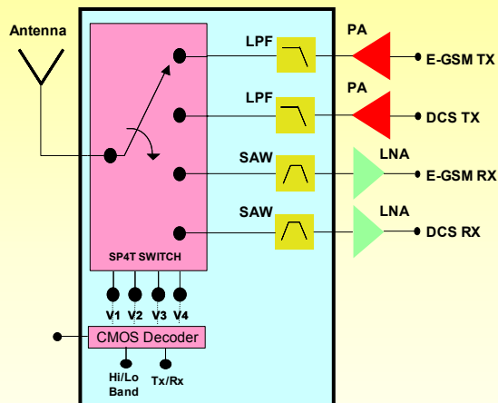
Dual Band GSM/DCS Antenna Switch Module TQP4M4004 Application
