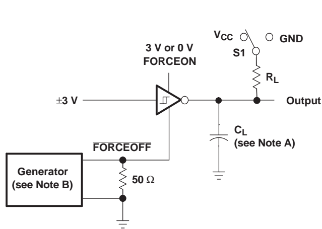
TEST CIRCUIT
