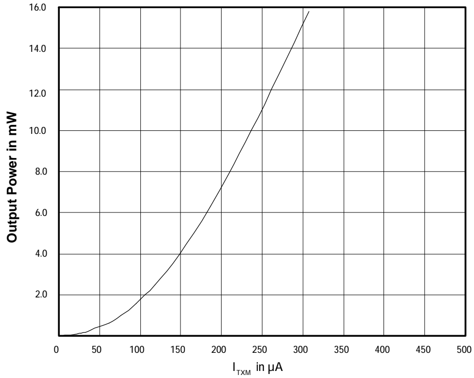
TR7000 RF Output Power vs I
