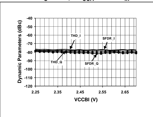
Figure 16. Distortion vs. V_{CCBI} F_S=20\text{MSPS} ; I_{CCA}=40\text{mA} ; F_{in}=5\text{MHz}
