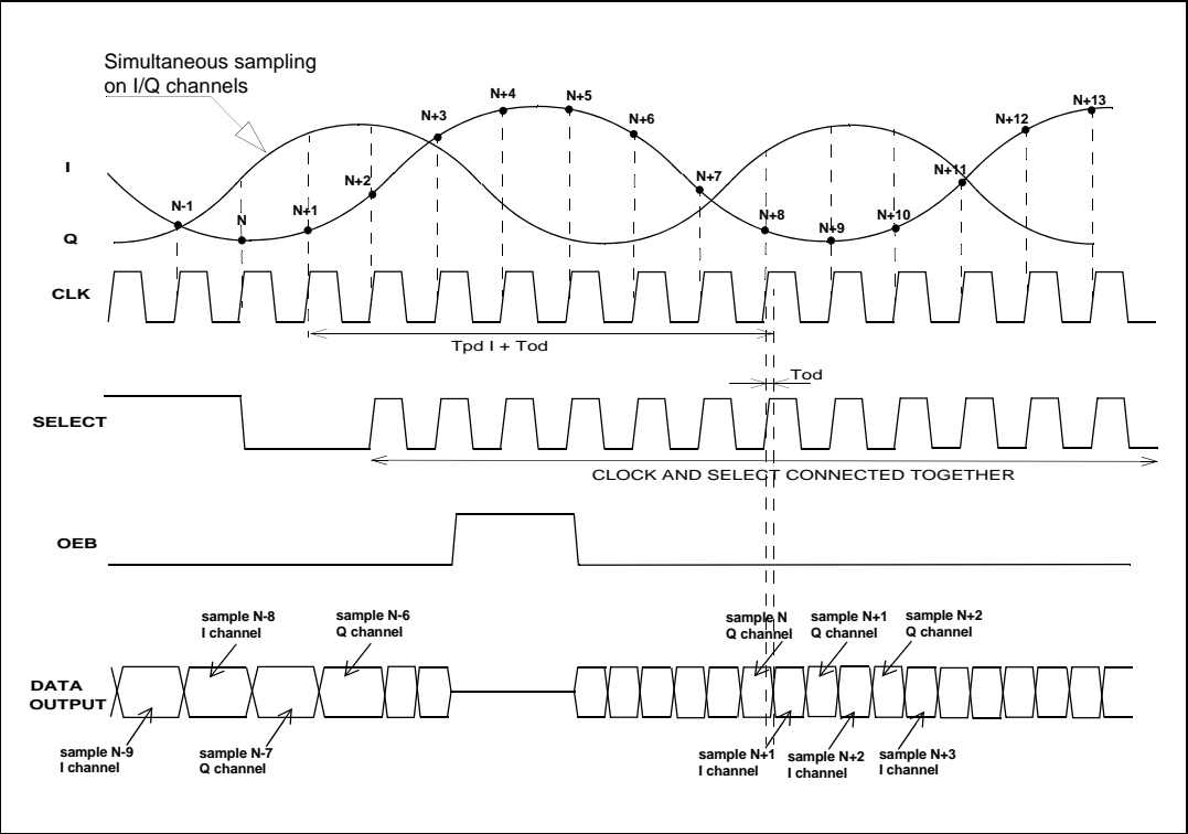
Figure 2. Timing diagram
