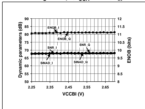
Figure 15. Linearity vs. V_{CCBI} F_S=20\text{MSPS} ; I_{CCA}=40\text{mA} ; F_{in}=5\text{MHz}
