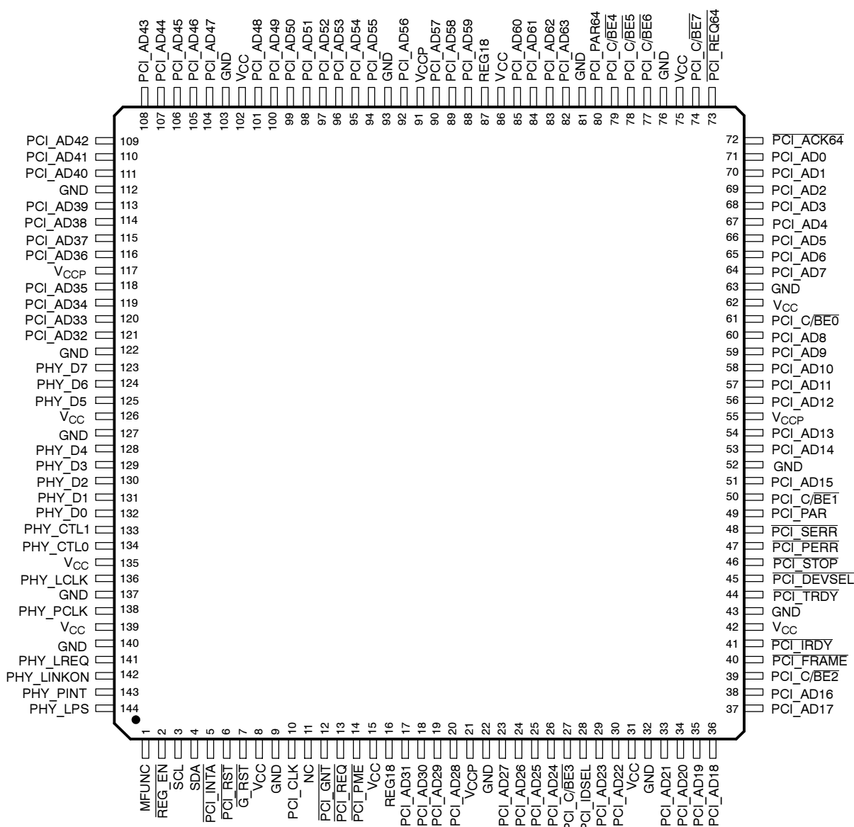
Figure 2-1. Terminal Assignments
