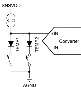
Figure 25. Functional Block Diagram of Temperature Measurement Mode
