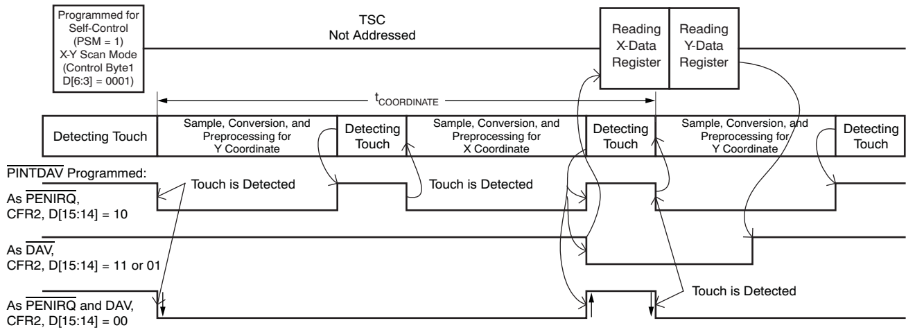
Figure 37. Example of an X and Y Coordinate Touch Screen Scan using TSMODE 1
