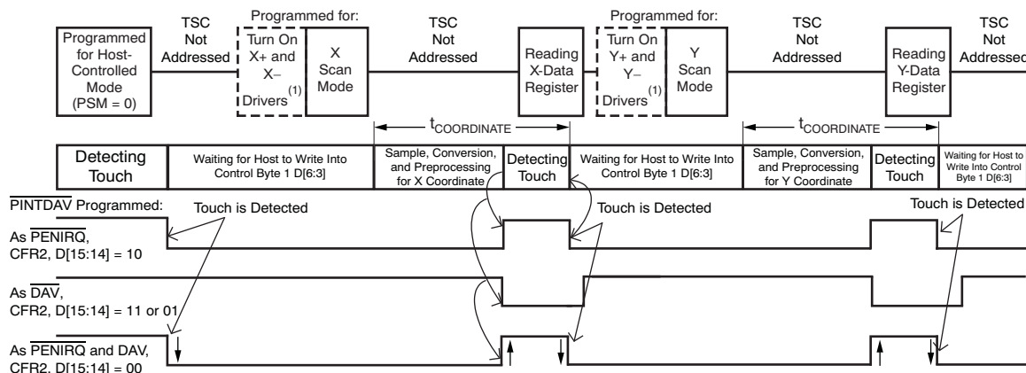
Figure 40. Example of X and Y Coordinate Touch Screen Scan using TSMODE 3
