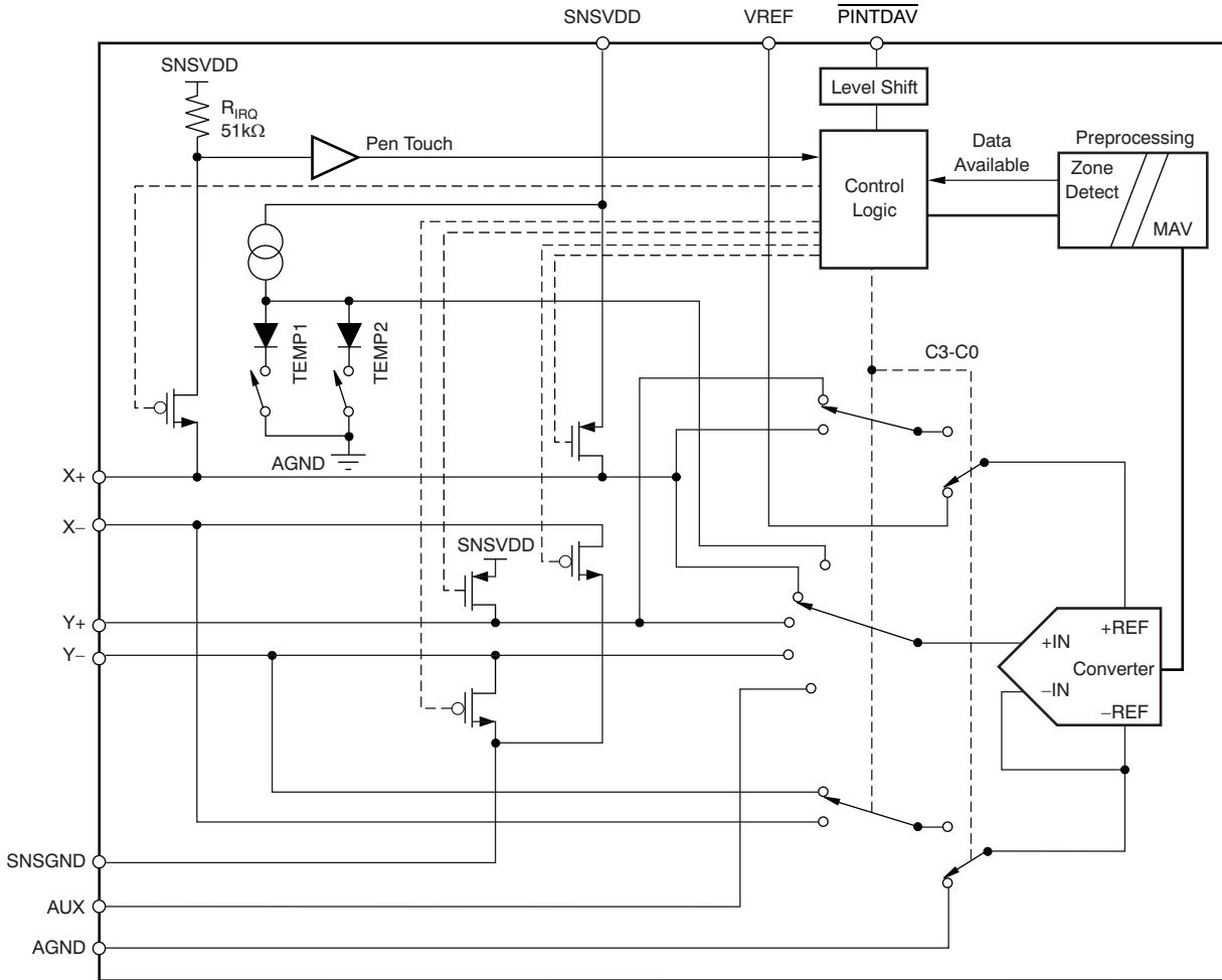
Figure 26. Simplified Diagram of the Analog Input Section
