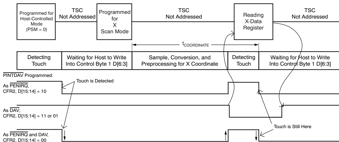
Figure 43. Example of a Single X Coordinate Touch Screen Scan (with Panel Stabilization Time) using TSMODE 3
