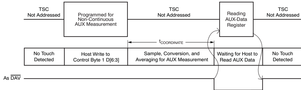
Figure 44. Non-Touch Screen, Non-Continuous AUX Measurement
