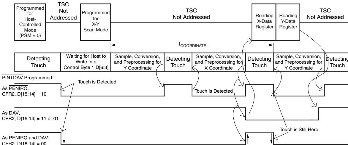
Figure 39. Example of an X and Y Coordinate Touch Screen Scan using TSMODE 2
