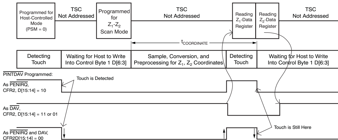
Figure 42. Example of a Z_1 and Z_2 Coordinate Touch Screen Scan (with Panel Stabilization Time) using TSMODE 3
