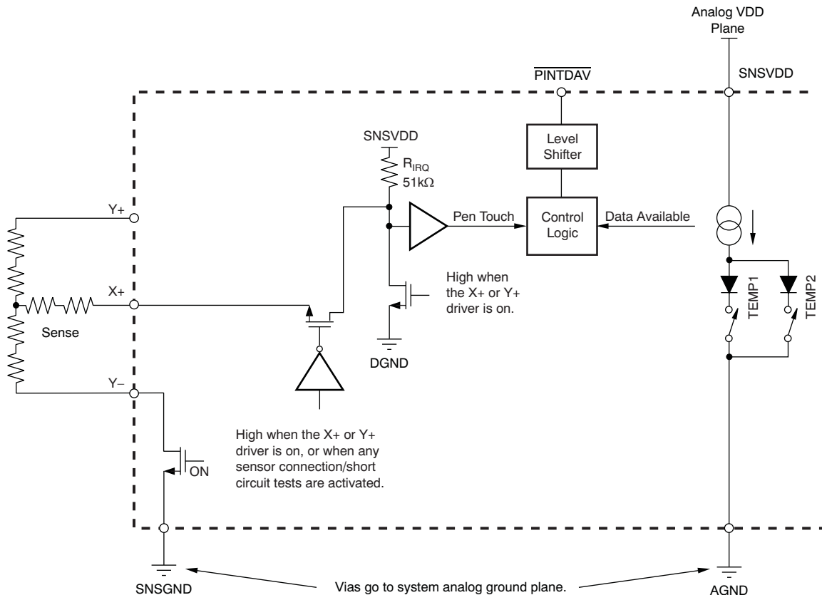
Figure 28. Example of a Pen-Touch Induced Interrupt via the \overline{\text{PINTDAV}} Pin
