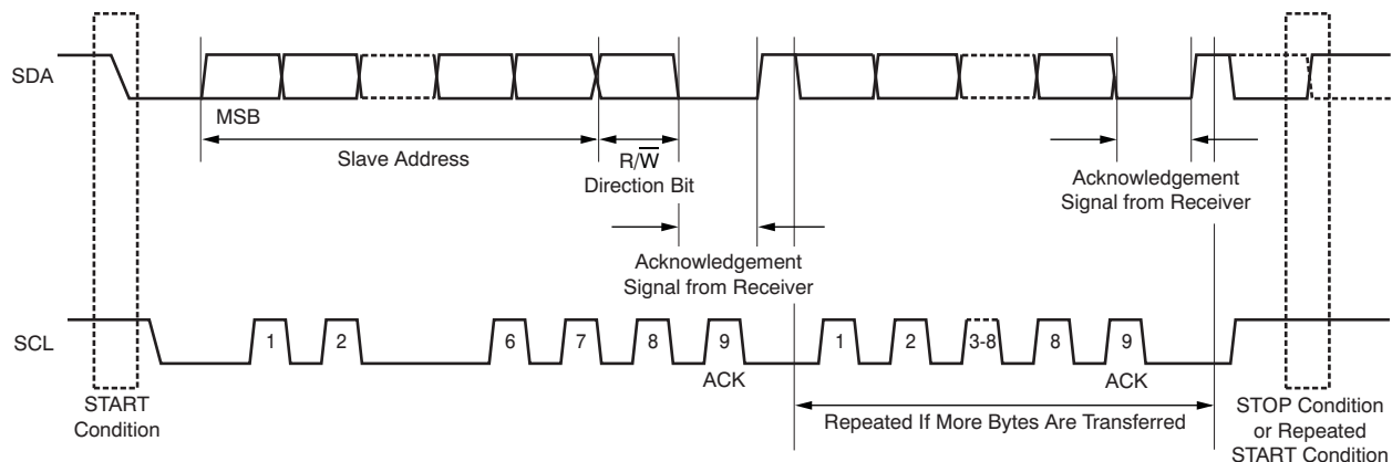
Figure 30. Complete Fast- or Standard-Mode Transfer
