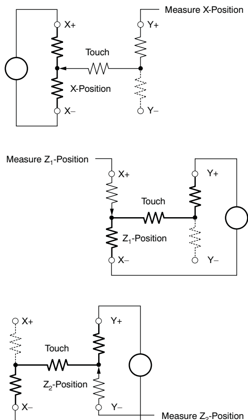
Figure 24. Pressure Measurement
