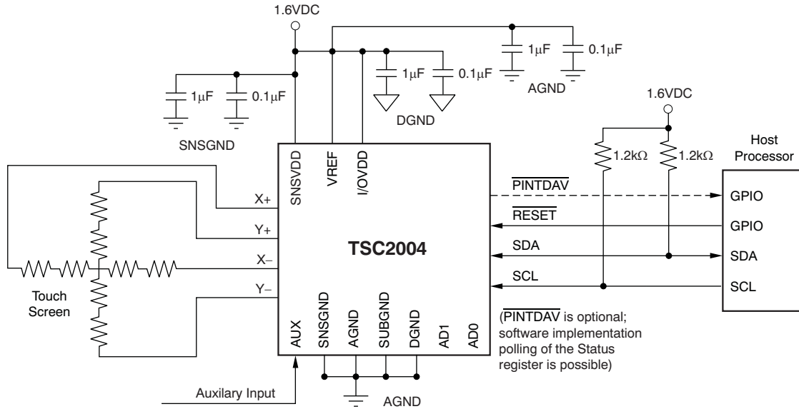
Figure 22. Typical Circuit Configuration
