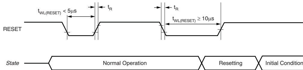
Figure 36. External Reset Timing
