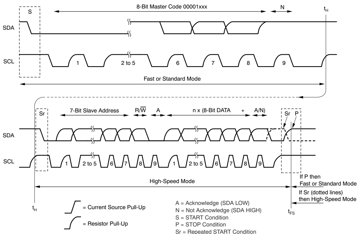
Figure 31. Complete High-Speed Mode Transfer
