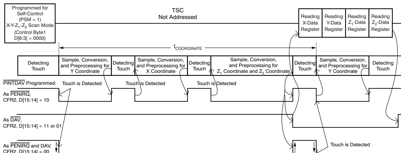
Figure 38. Example of an X, Y, and Z Coordinate Touch Screen Scan using TSMODE 1
