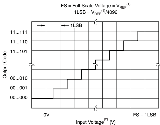
Figure 27. Ideal Input Voltages and Output Codes
