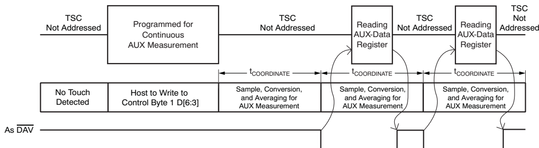
Figure 45. Non-Touch Screen, Continuous AUX Measurement
