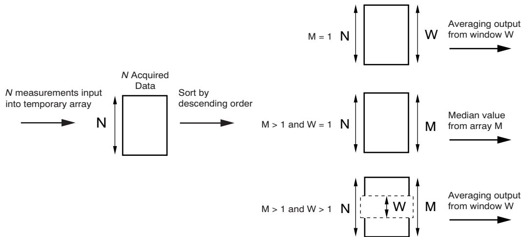
Figure 29. MAV Filter Operation (patent pending)
