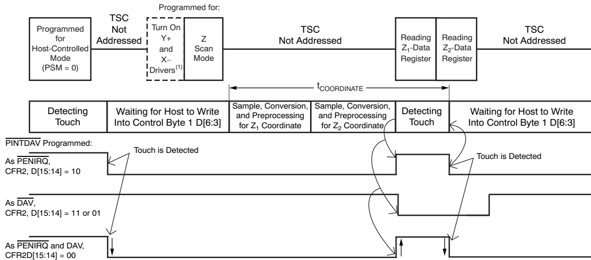
Figure 41. Example of Z_1 and Z_2 Coordinate Touch Screen Scan (without Panel Stabilization Time) using TSMODE 3
