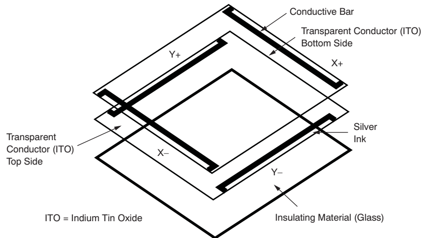
Figure 23. 4-Wire Touch Screen Construction
