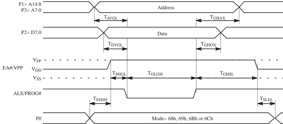
Figure 24. EPROM Programming Waveforms
