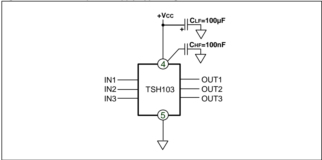
Figure 7. Circuit for power supply bypassing
