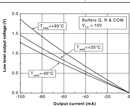
Figure 19. Voltage output low ( V_{OL} ) vs. output current - buffer Q, R & COM
