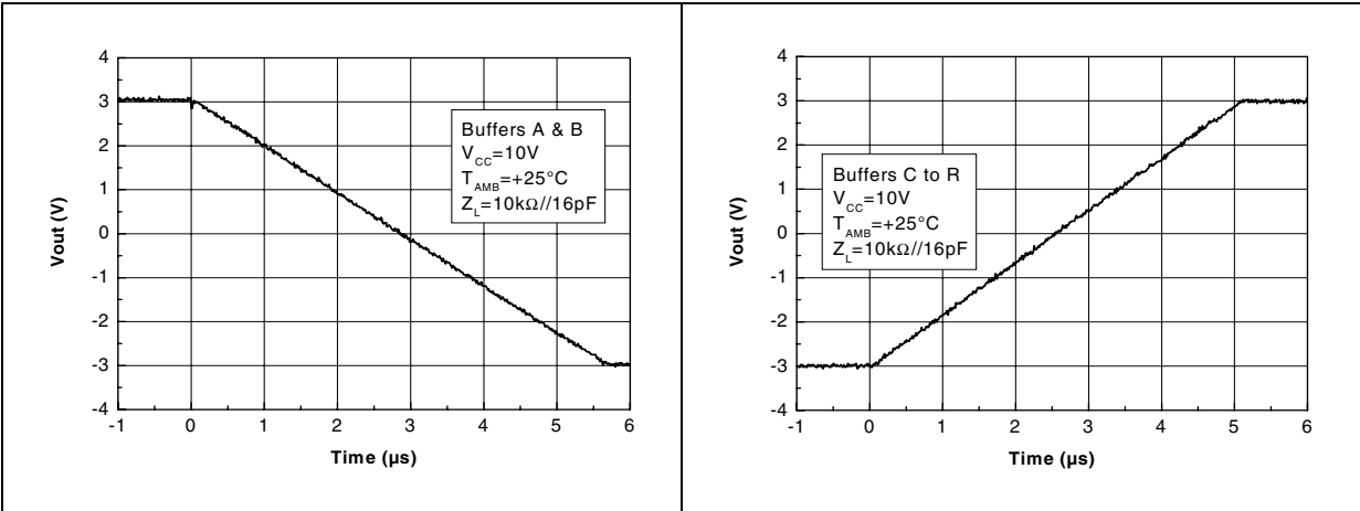
Figure 28. Large signal response - buffers A & B Figure 29. Large signal response - buffers C to R
