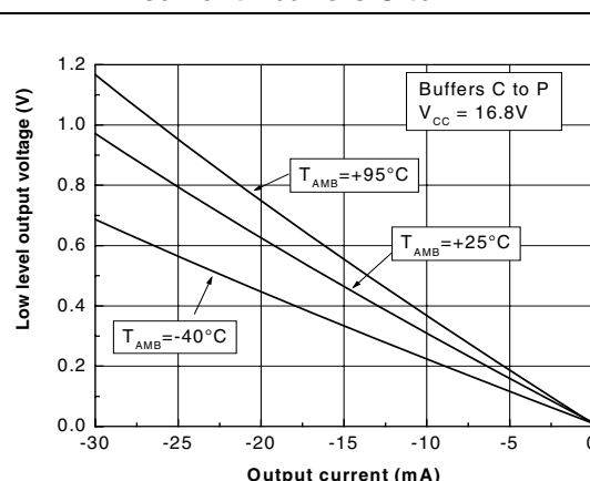
Figure 17. Voltage output low ( V_{OL} ) vs. output current - buffers C to P
