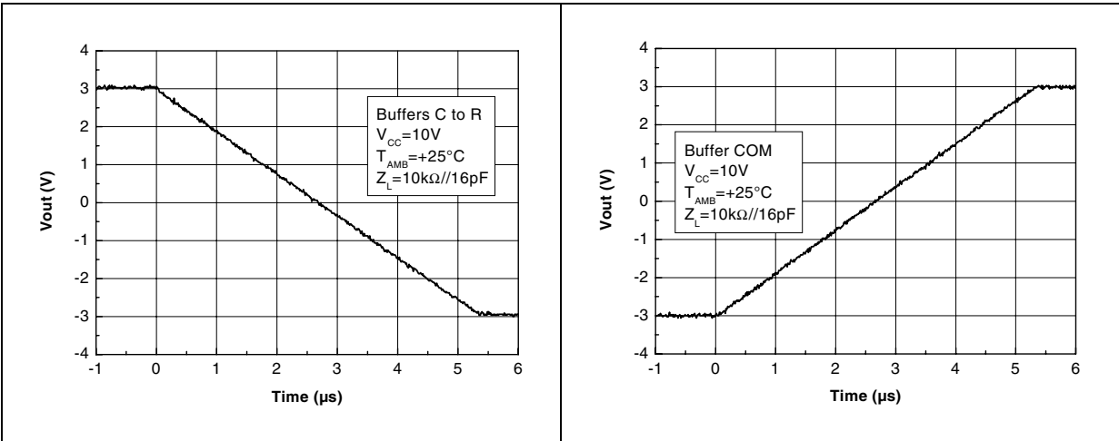
Figure 30. Large signal response - buffers C to R Figure 31. Large signal response - buffer COM
