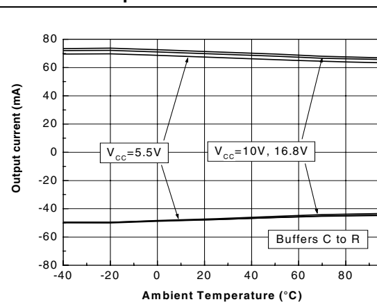
Figure 7. Output current capability vs. temperature
