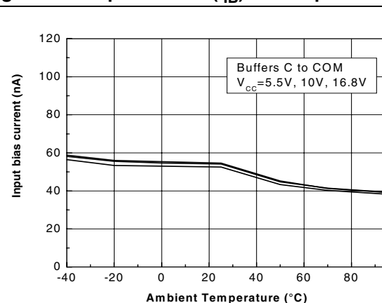
Figure 5. Input current ( I_{IB} ) vs. temperature
