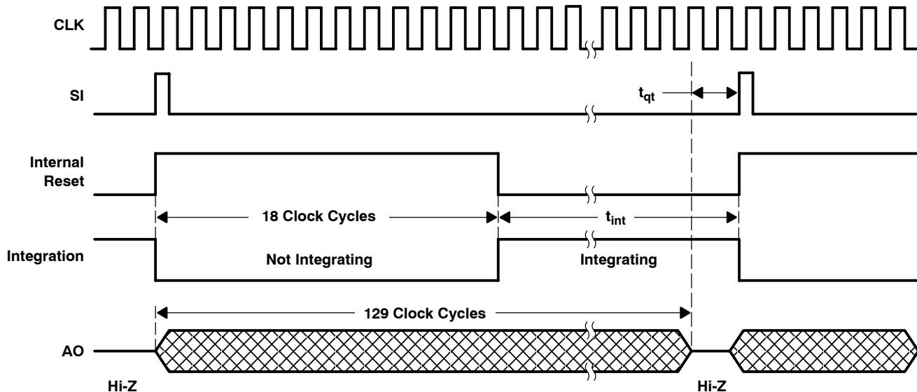
Figure 1. Timing Waveforms
