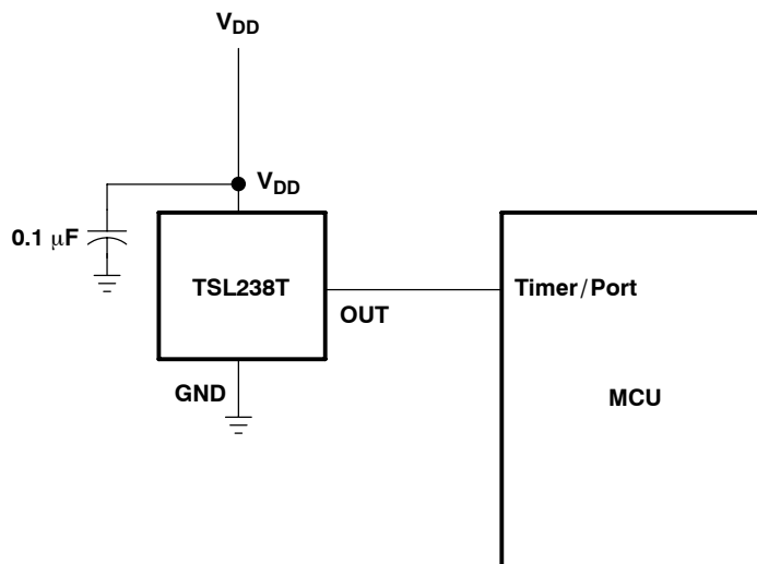
Figure 8. Typical TSL238T Interface to a Microcontroller
