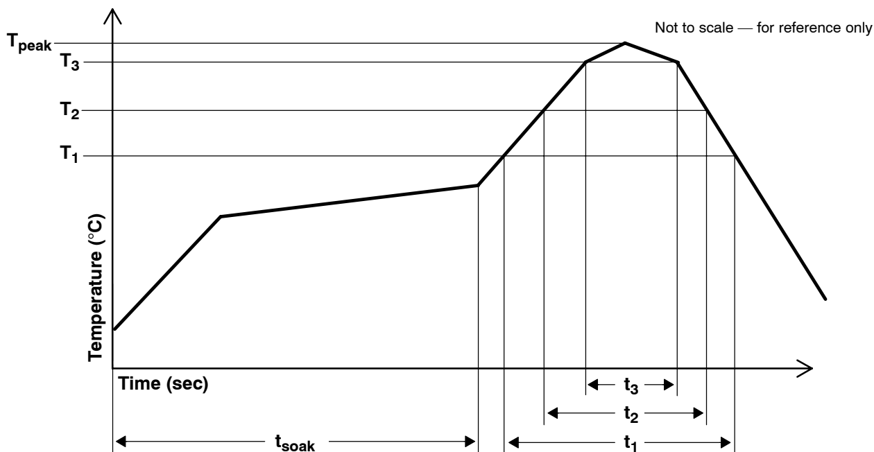
Figure 12. TSL238T Solder Reflow Profile
