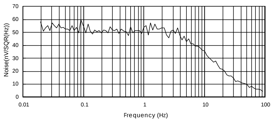
Noise = F(frequency)
