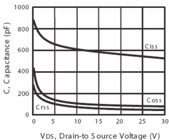
Figure 3. Capacitance
