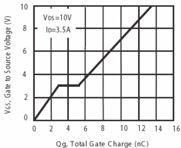
Figure 9. Gate Charge
