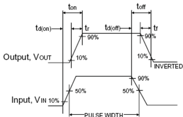
Switchin Waveforms
