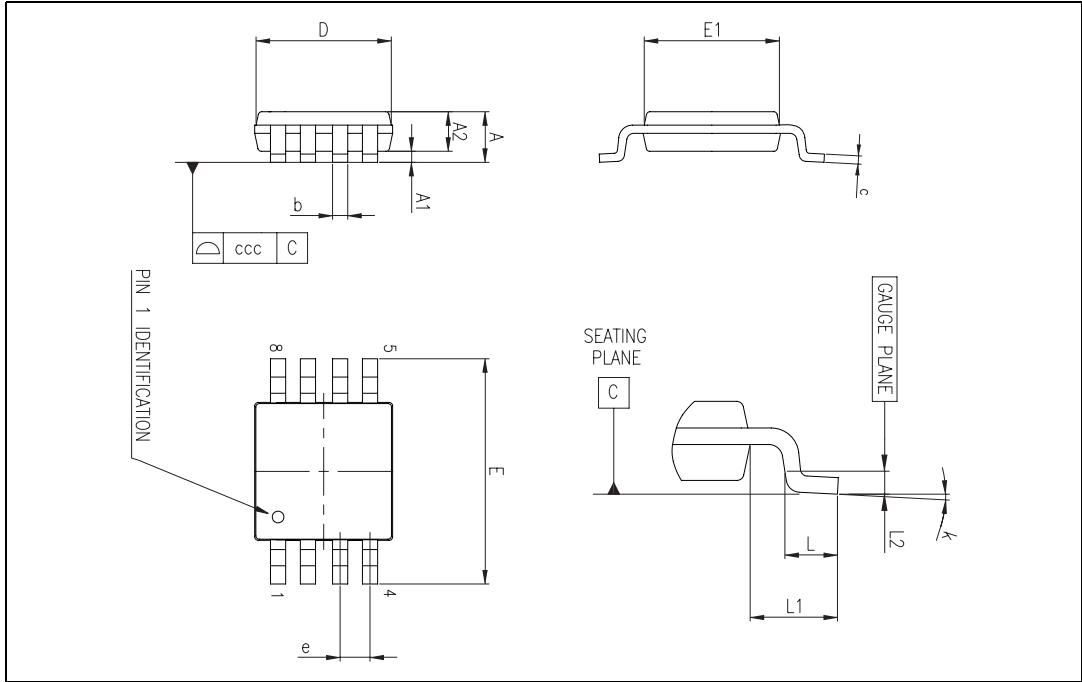
Figure 52. MiniSO-8 package mechanical drawing
