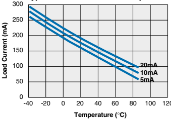
TS190 Typical Load Current vs. Temperature
