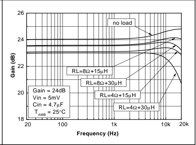
Figure 17. Gain vs. frequency
