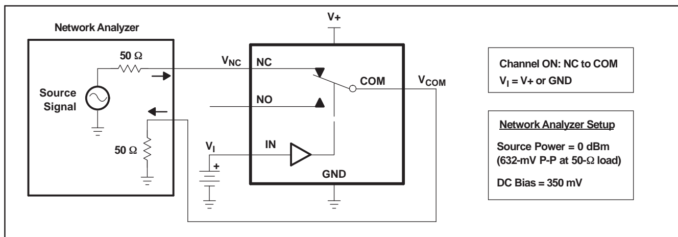
Figure 16. Bandwidth (BW)
