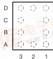
YZP PACKAGE TERMINAL ASSIGNMENTS
