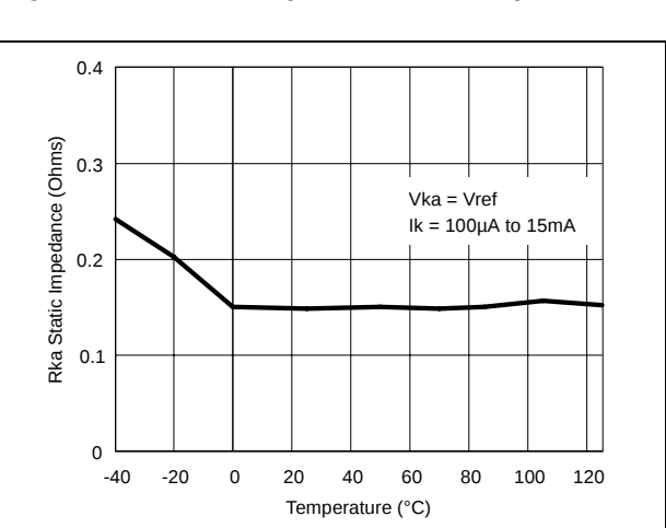
Figure 7. Static impedance vs. temperature
