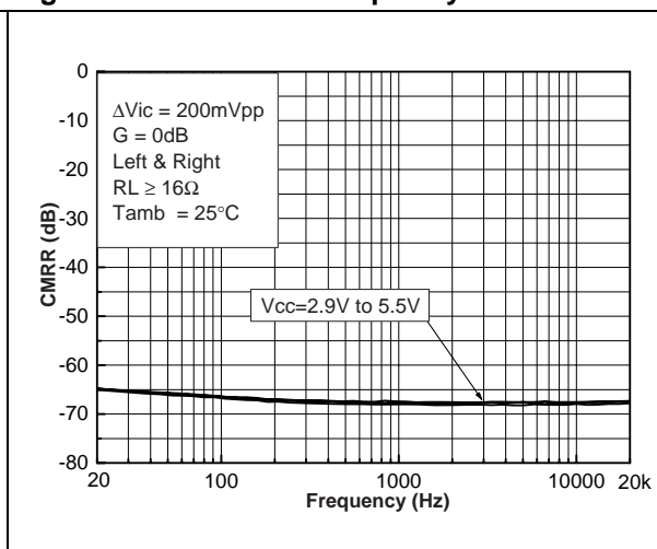
Figure 41. CMRR vs. frequency
