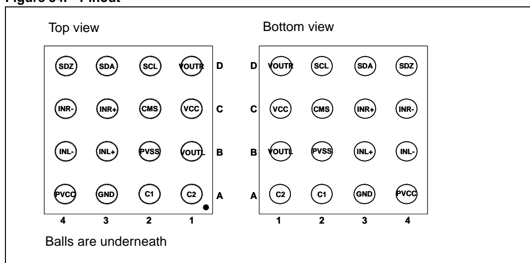
Figure 54. Pinout
