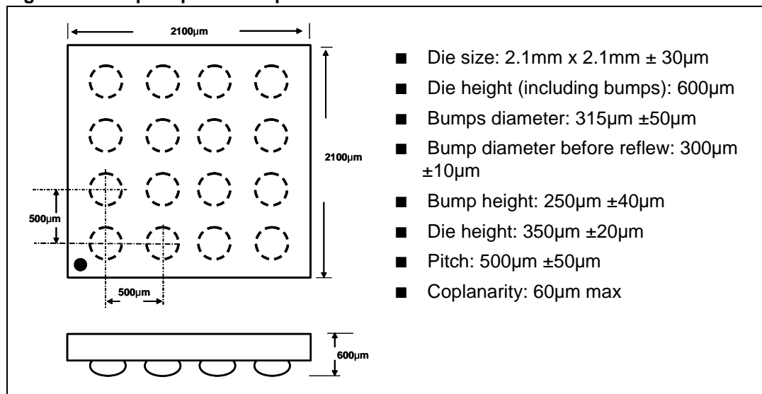
Figure 56. Flip-chip - 16 bumps
