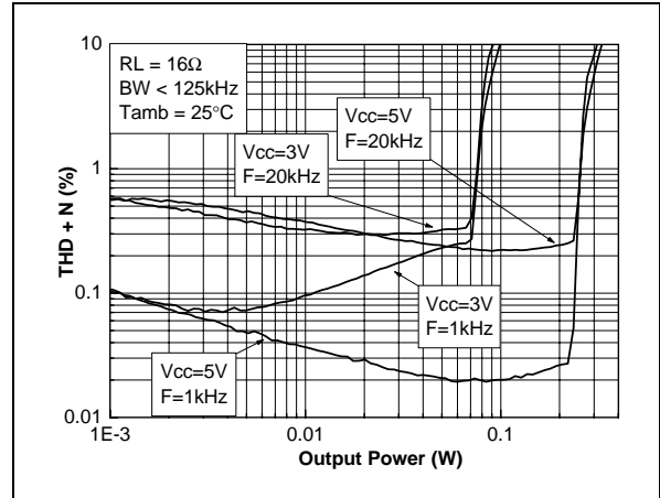
Figure 5: HDout THD+N vs. output power (Output modes 2, 3 G=+3dB)
