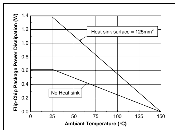
Figure 42: Power derating curves
