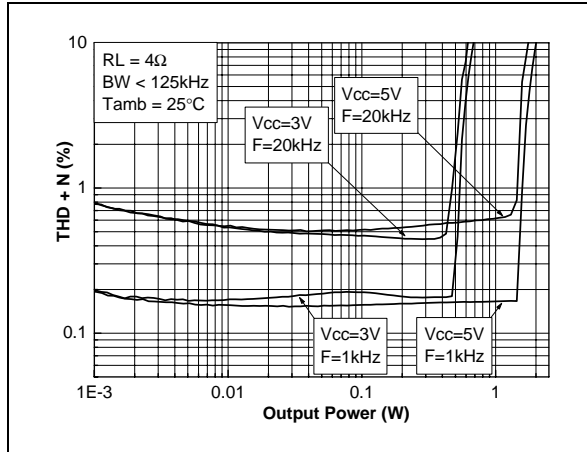
Figure 2: Spkout THD+N vs. output power (Output modes 1, 3, 5, 7)
