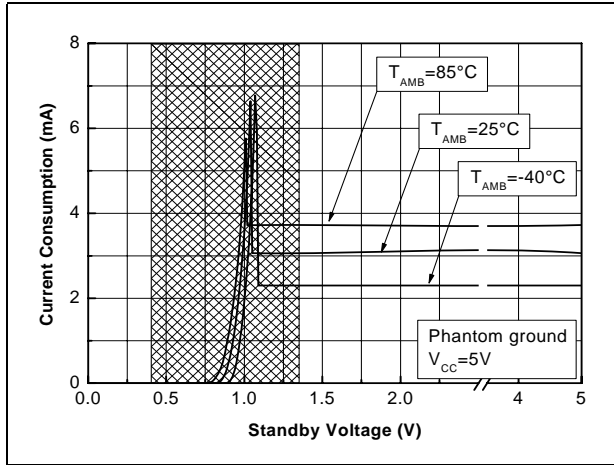
Figure 74. Current consumption vs. standby voltage
